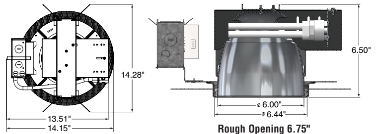
XB - Cross Blade Louver
